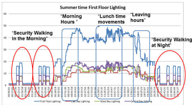
Figure 2: Behavioural anomalies observed in energy consumption of the lighting subsystem.
